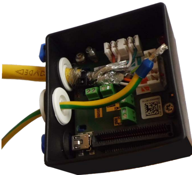
Fig. 28: Ground wire inserted, plug properly seated
