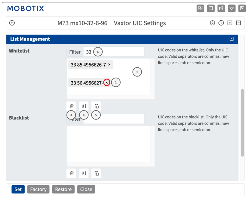
Fig. 7: Black and white lists
