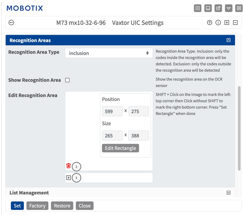
Fig. 6: Recognition Areas
