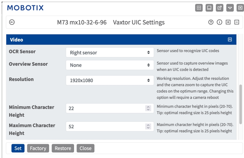
Fig. 8: Video
