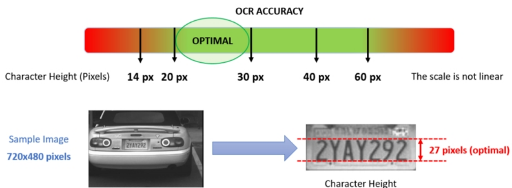
Fig. 2: Minimum character height
