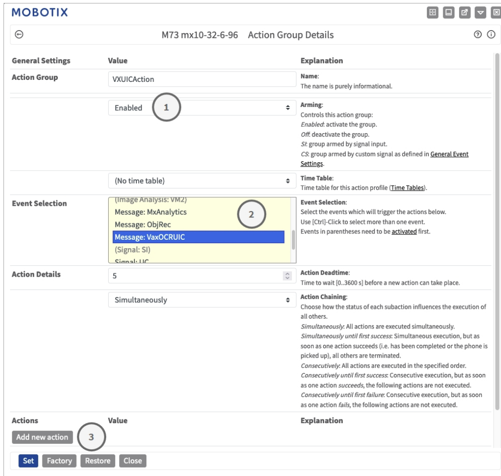
Fig. 13: Configuring an Action Group
