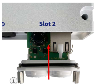
Fig. 6: Conexión del S74 Network Slide in Board with RJ45 socket
