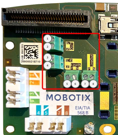
Conectores de terminal, Connector Box LSA
