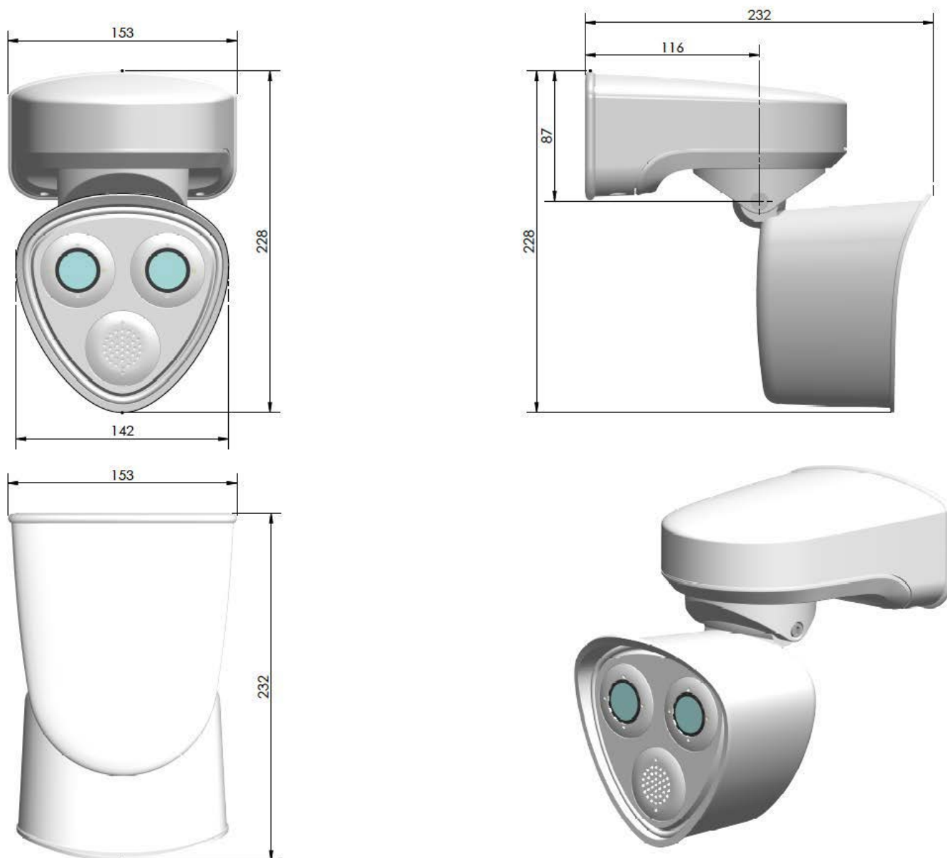
Fig. 4: MOBOTIX M73: All measurements in mm
