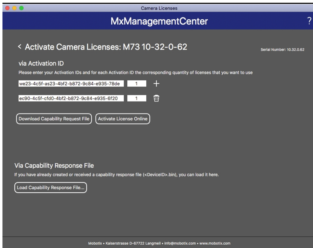
Fig. 3: Adding licenses
