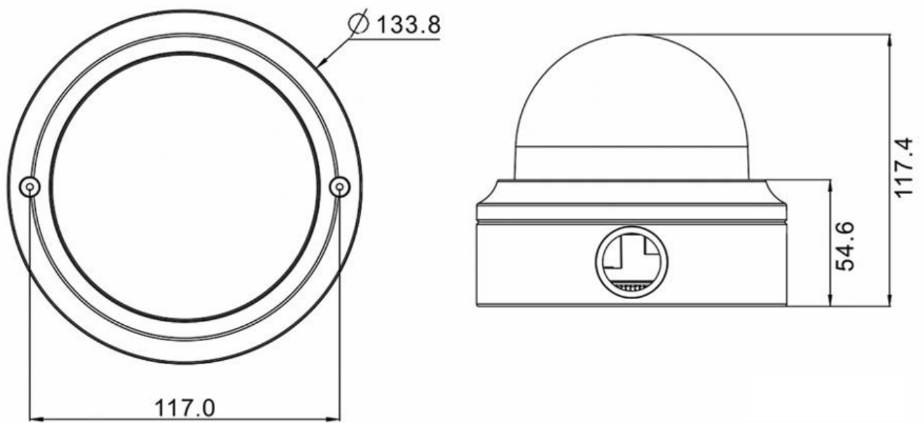
Abb. 1: 5MP Vandal Fixed Dome Analytics Camera: Alle Maße in mm
