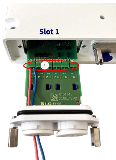
Fig. 19: IO wires connected to terminal
