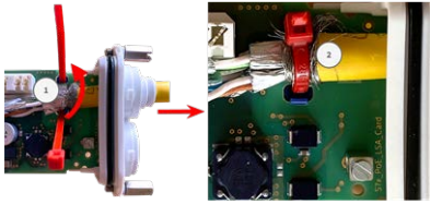
Fig. 11: Cable tie inserted beneath network cable
