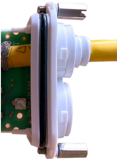
Fig. 10: Network cable inserted, plug properly seated
