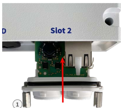
Fig. 6: Connecting the S74 Network Slide in Board with RJ45 socket
