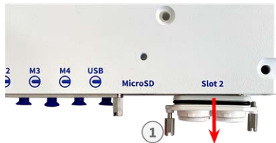
Fig. 5: Remove cover from interface board slot
