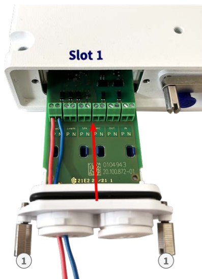
Fig. 20: Connecting the S74 Network Slide in Board with RJ45 socket
