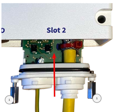
Fig. 16: Connecting the S74 Network Slide in Board with LSA terminal
